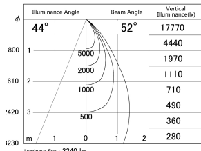
■ Direct Horizontal Illuminance DD155-3055MB9027
