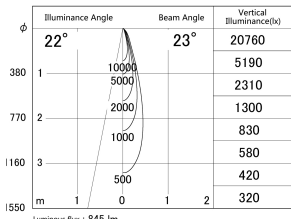
■ Direct Horizontal Illuminance DD155-0825MB9030
