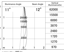
■ Direct Horizontal Illuminance DD155-1010MB9030
