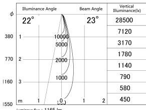
■ Direct Horizontal Illuminance DD155-1025MB9030
