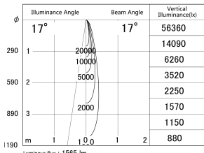
■ Direct Horizontal Illuminance DD155-1515MB9030
