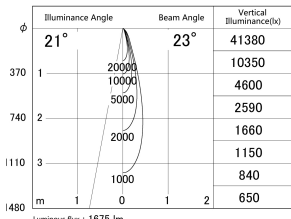
■ Direct Horizontal Illuminance DD155-1525MB9030
