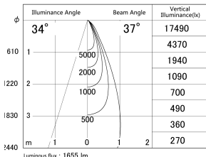
■ Direct Horizontal Illuminance DD155-1535MB9030
