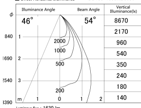
■ Direct Horizontal Illuminance DD155-1555MB9030
