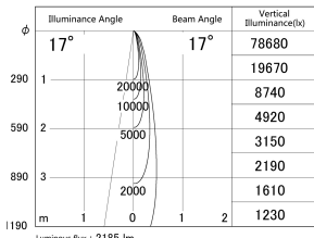
■ Direct Horizontal Illuminance DD155-2015MB9030
