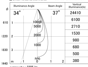
■ Direct Horizontal Illuminance DD155-2035MB9030
