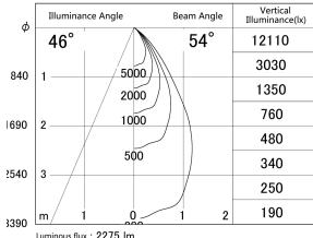
■ Direct Horizontal Illuminance DD155-2055MB9030
