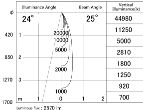
■ Direct Horizontal Illuminance DD155-2525MB9030
