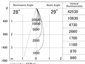
■ Direct Horizontal Illuminance DD155-2530MB9030
