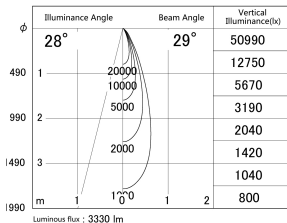
■ Direct Horizontal Illuminance DD155-3030MB9030
