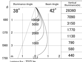
■ Direct Horizontal Illuminance DD155-3040MB9030
