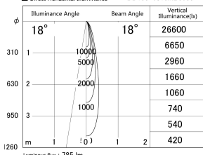
■ Direct Horizontal Illuminance DD155-0815MB9035
