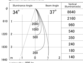
■ Direct Horizontal Illuminance DD155-0835MB9035
