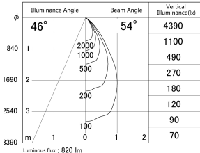
■ Direct Horizontal Illuminance DD155-0855MB9035
