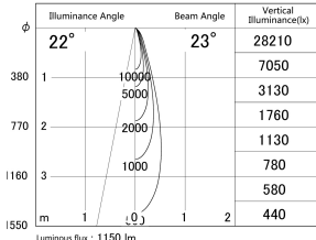
■ Direct Horizontal Illuminance DD155-1025MB9035
