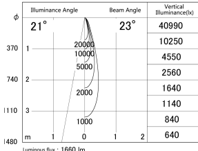
■ Direct Horizontal Illuminance DD155-1525MB9035
