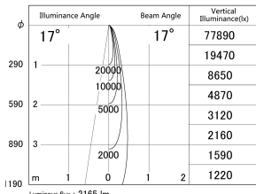
■ Direct Horizontal Illuminance DD155-2015MB9035
