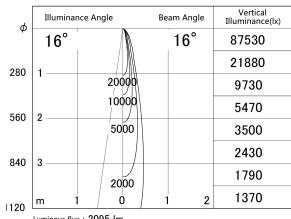
■ Direct Horizontal Illuminance DD155-2515MB9035
