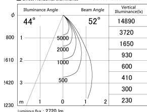
■ Direct Horizontal Illuminance DD155-2555MB9035
