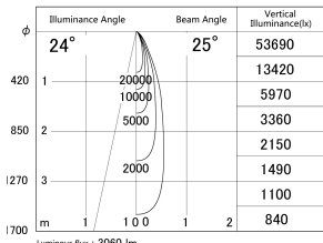
■ Direct Horizontal Illuminance DD155-3025MB9035
