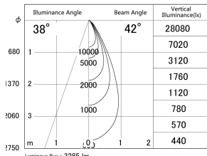
■ Direct Horizontal Illuminance DD155-3040MB9035
