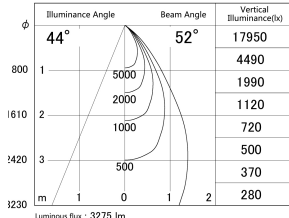
■ Direct Horizontal Illuminance DD155-3055MB9035
