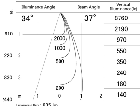
■ Direct Horizontal Illuminance DD155-0835MB9040
