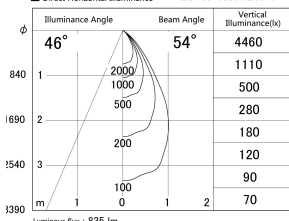
■ Direct Horizontal Illuminance DD155-0855MB9040
