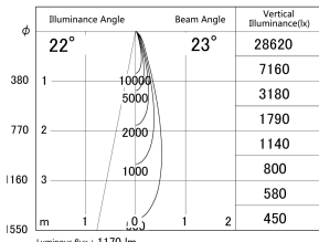
■ Direct Horizontal Illuminance DD155-1025MB9040
