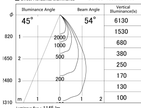
■ Direct Horizontal Illuminance DD155-1055MB9040
