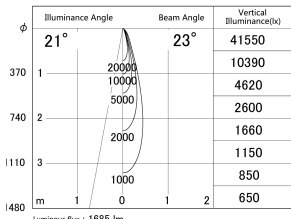
■ Direct Horizontal Illuminance DD155-1525MB9040
