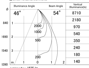
■ Direct Horizontal Illuminance DD155-1555MB9040
