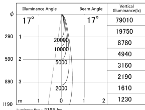
■ Direct Horizontal Illuminance DD155-2015MB9040
