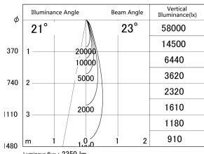
■ Direct Horizontal Illuminance DD155-2025MB9040
