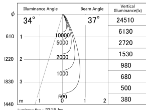
■ Direct Horizontal Illuminance DD155-2035MB9040
