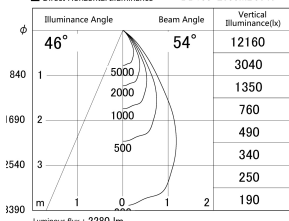
■ Direct Horizontal Illuminance DD155-2055MB9040
