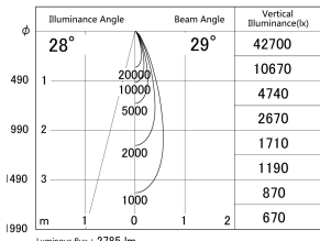
■ Direct Horizontal Illuminance DD155-2530MB9040
