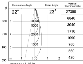
■ Direct Horizontal Illuminance DD155-1025DW9027
