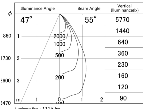
■ Direct Horizontal Illuminance DD155-1055DW9027
