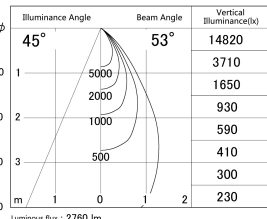
■ Direct Horizontal Illuminance DD155-2555DW9027
