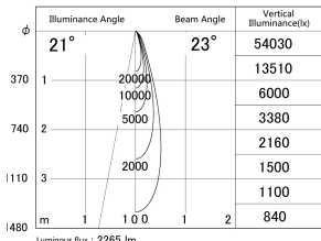
■ Direct Horizontal Illuminance DD155-2025DW9030
