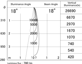
■ Direct Horizontal Illuminance DD155-0815DW9035
