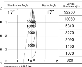
■ Direct Horizontal Illuminance DD155-1515DW9035
