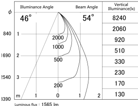
■ Direct Horizontal Illuminance DD155-1555DW9035
