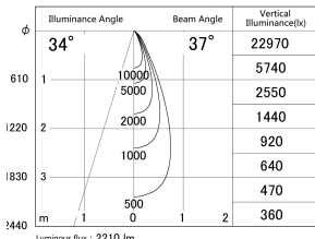
■ Direct Horizontal Illuminance DD155-2035DW9035
