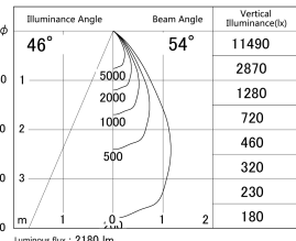
■ Direct Horizontal Illuminance DD155-2055DW9035
