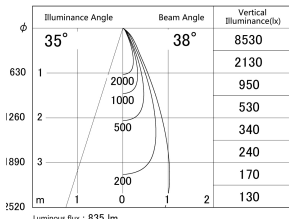
■ Direct Horizontal Illuminance DD155-0835DW9040
