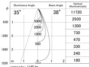
■ Direct Horizontal Illuminance DD155-1035DW9040
