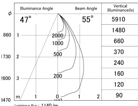
■ Direct Horizontal Illuminance DD155-1055DW9040
