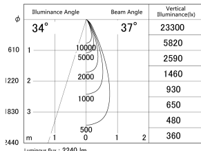
■ Direct Horizontal Illuminance DD155-2035DW9040
